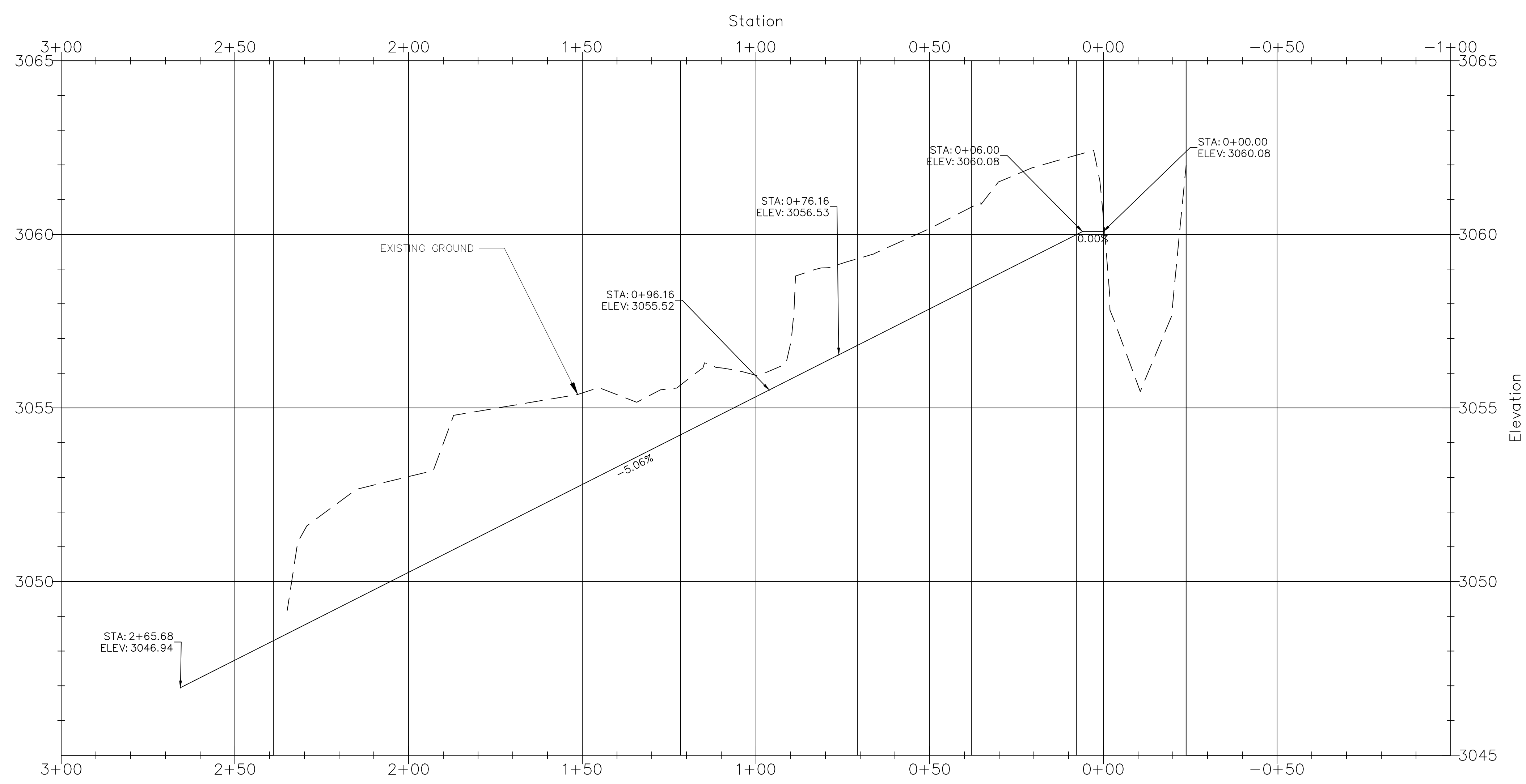
Overflow Channel Profile
